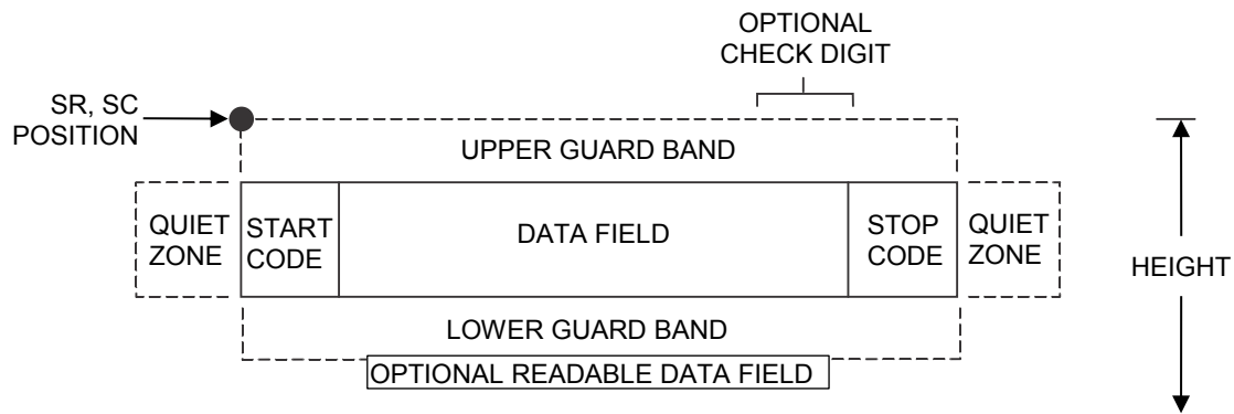
Figure 25 UPS 11 Structure
